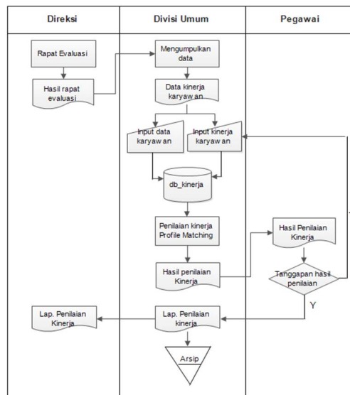
Gambar 2 Diagram Alir Dokumen (Flowmap)
